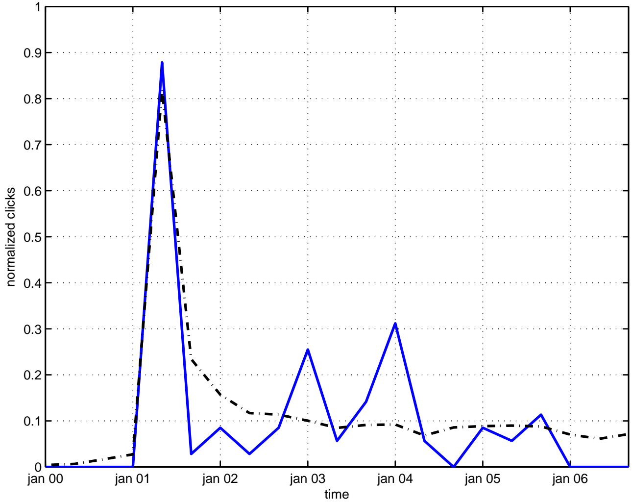
classical trajectory
