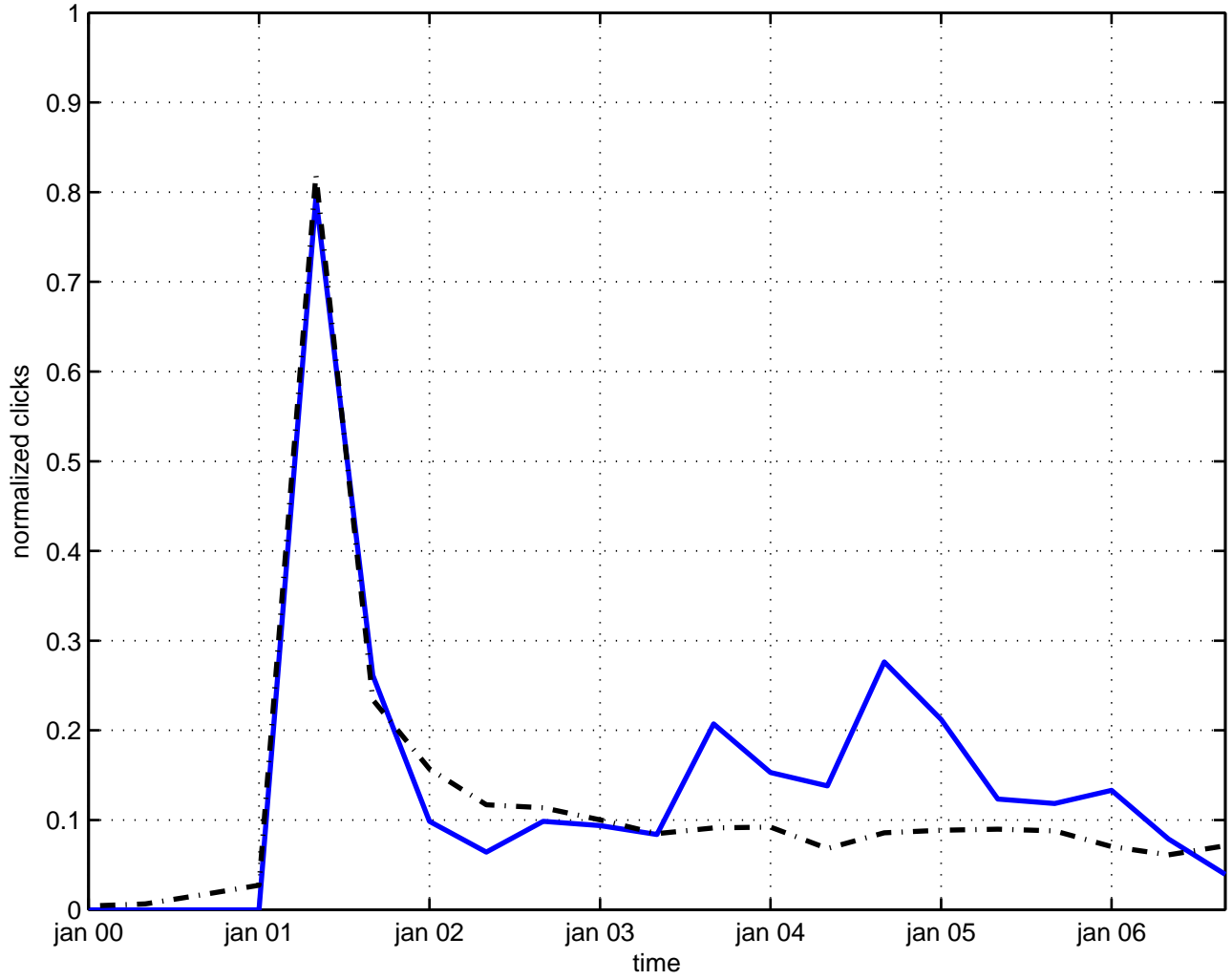
classical potential
