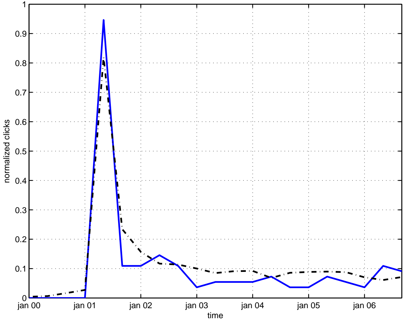
classical master equation
