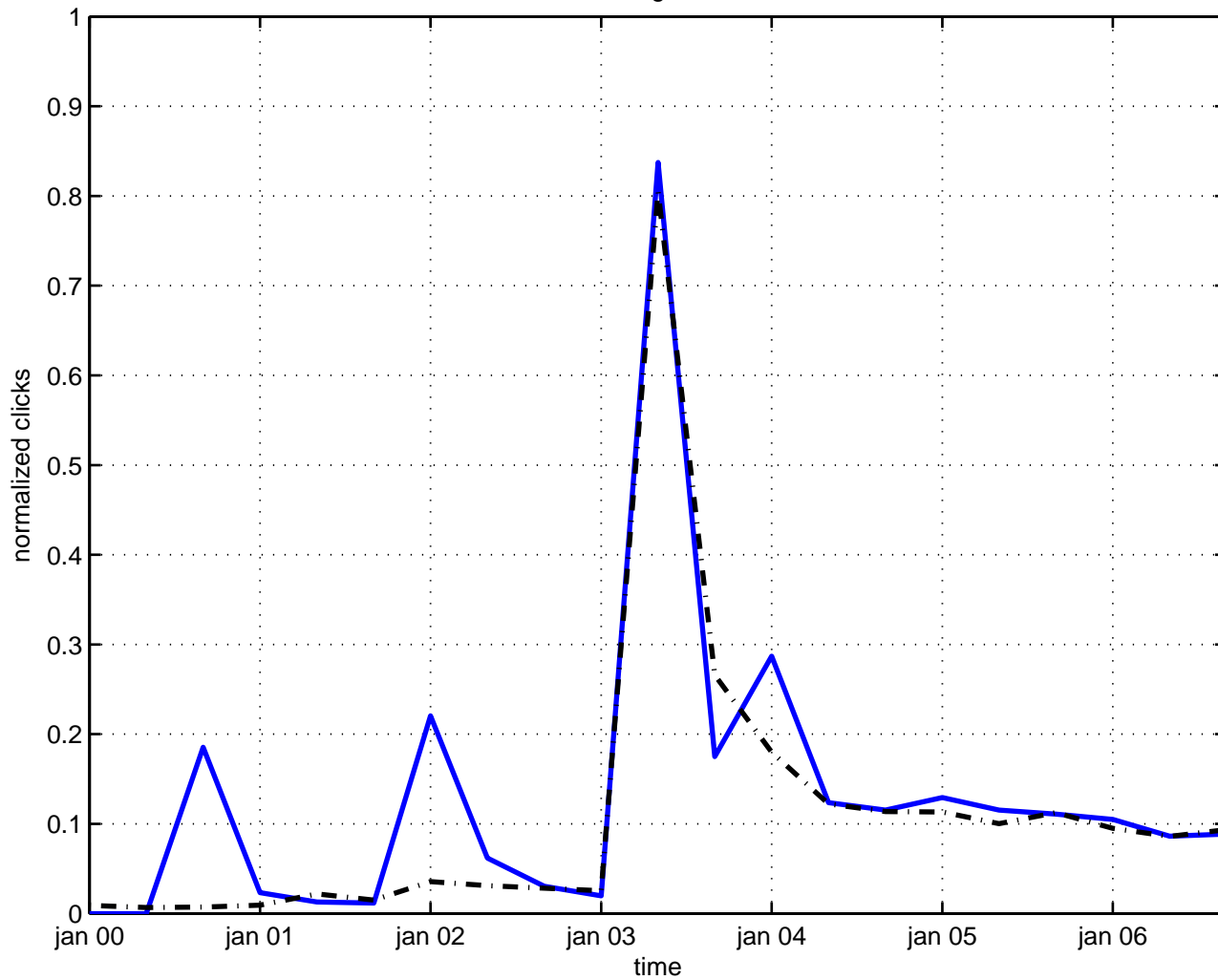
classical gravitation
