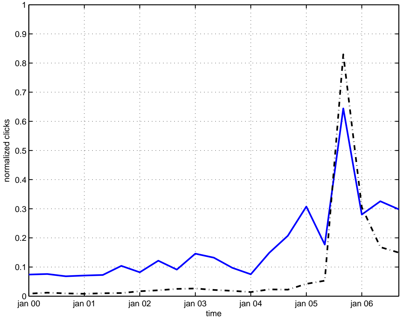
classical field theory
