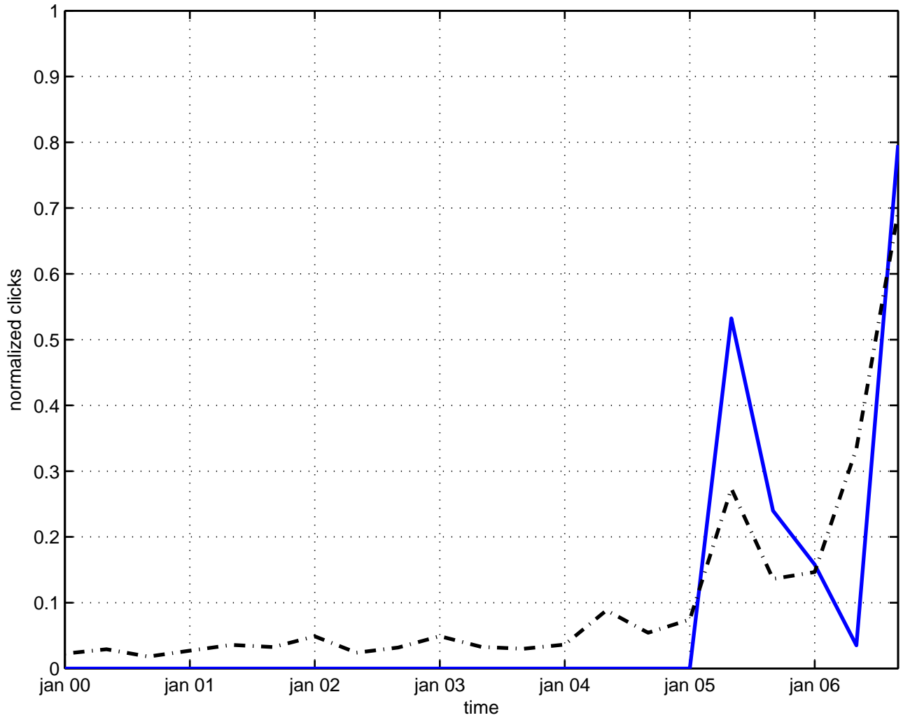
ckm matrix
