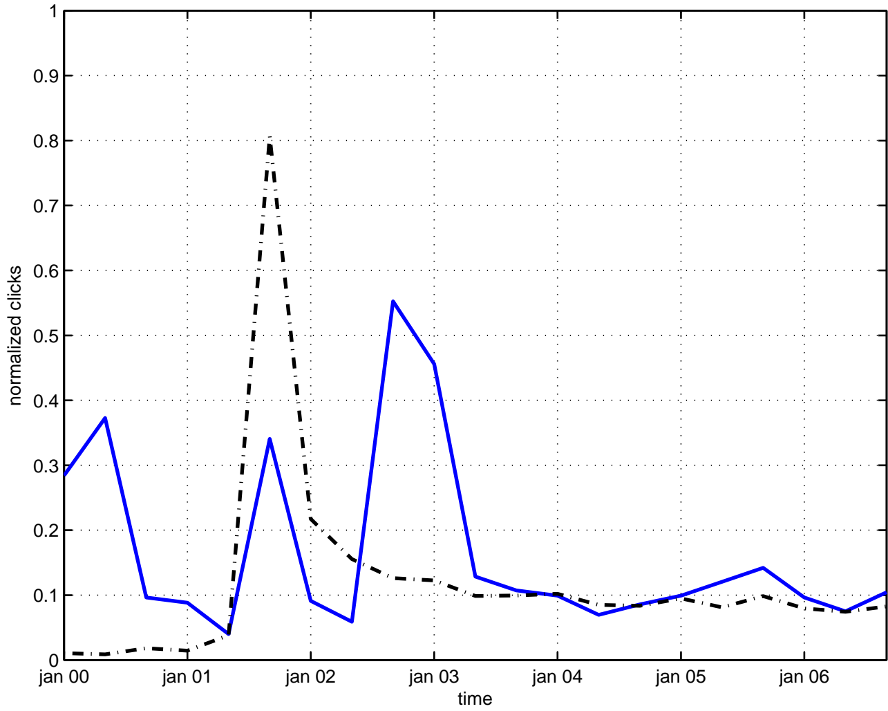
chiral wess-zumino-witten model
