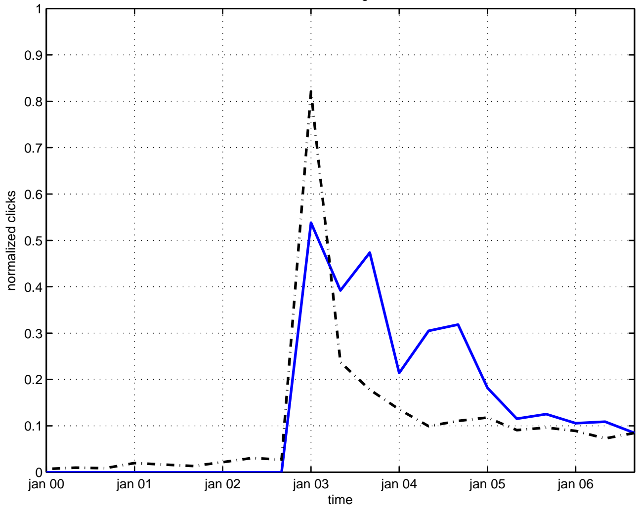
chiral ring
