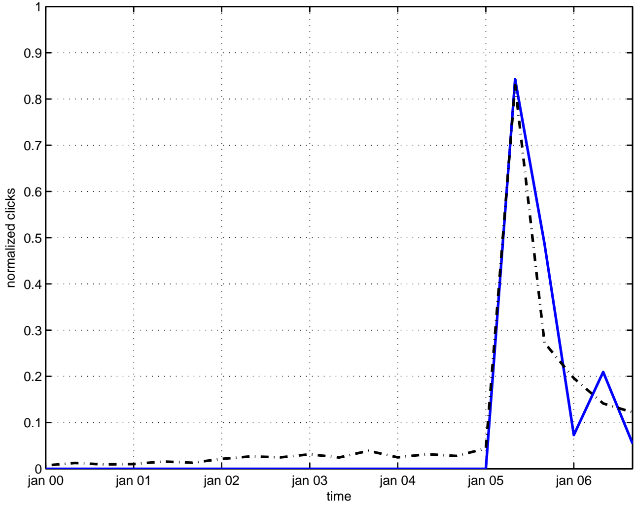
chiral r parity
