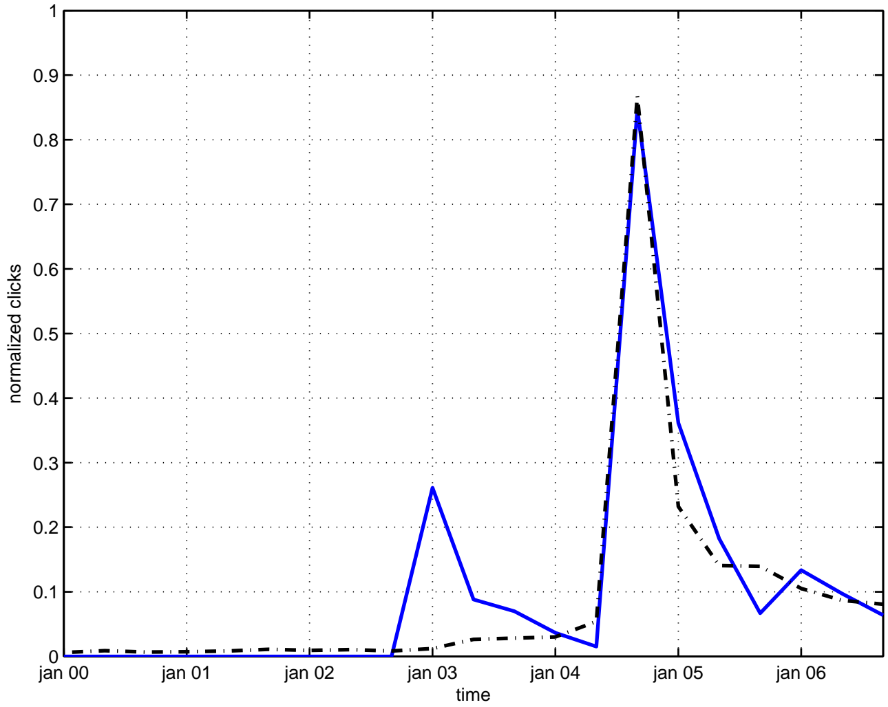
chiral gravitation
