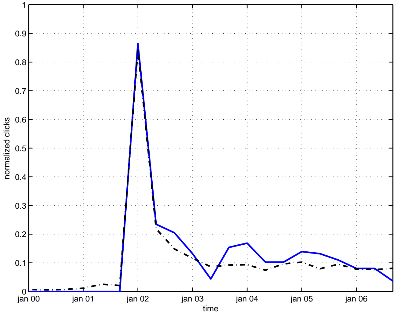
chiral bosonization
