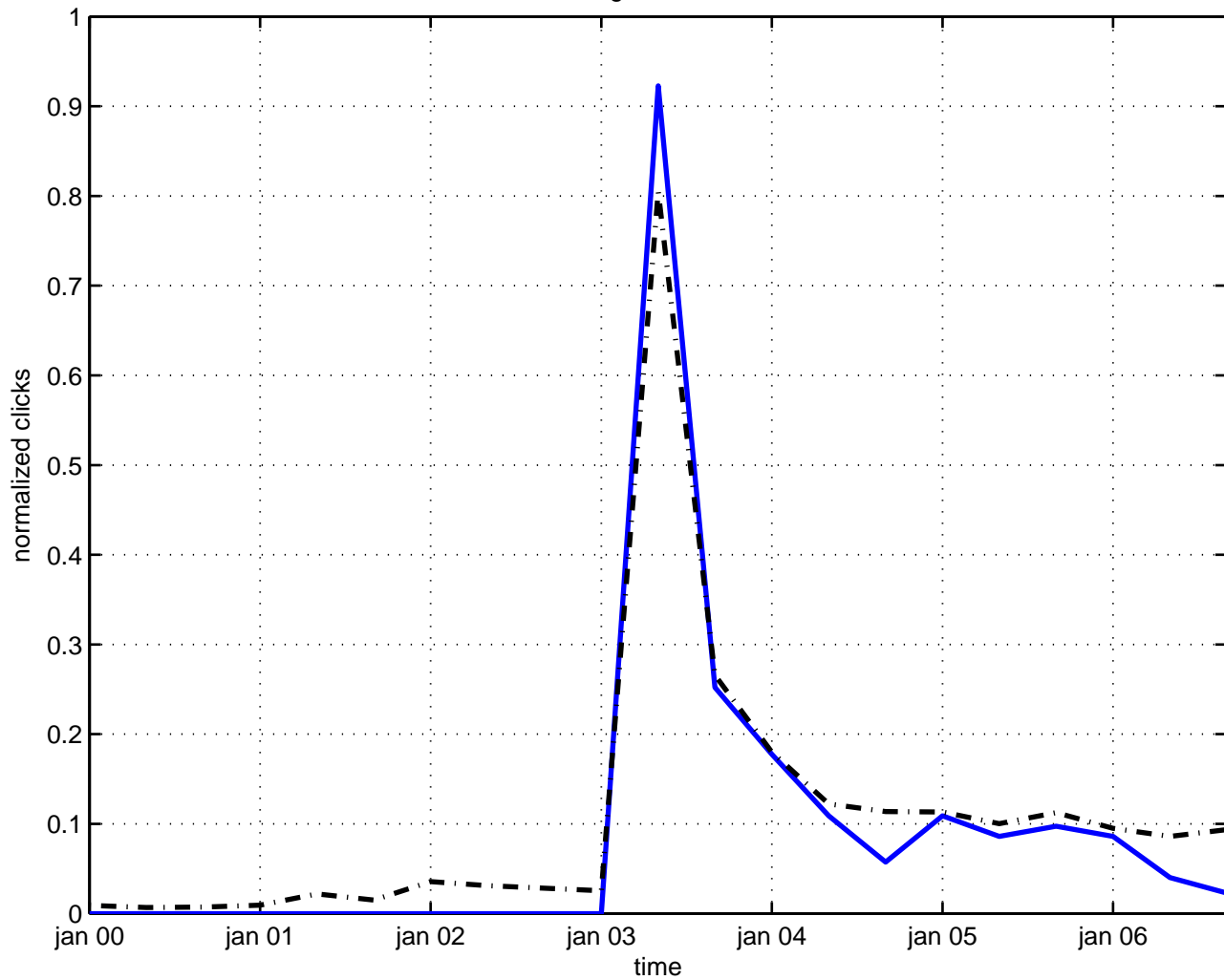
charge wormhole
