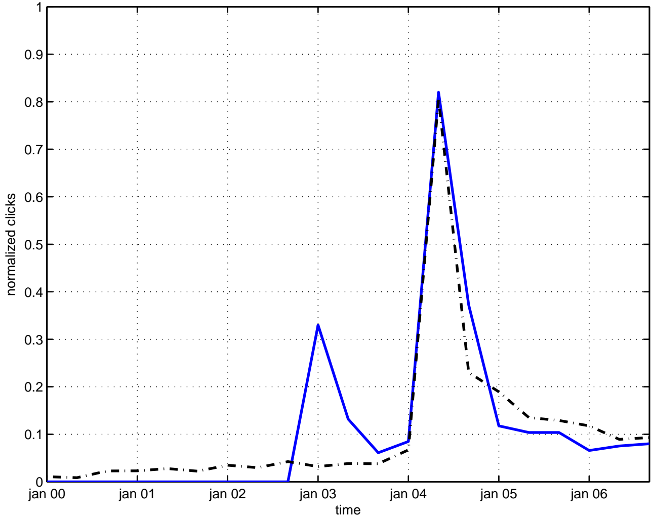
charge q-ball
