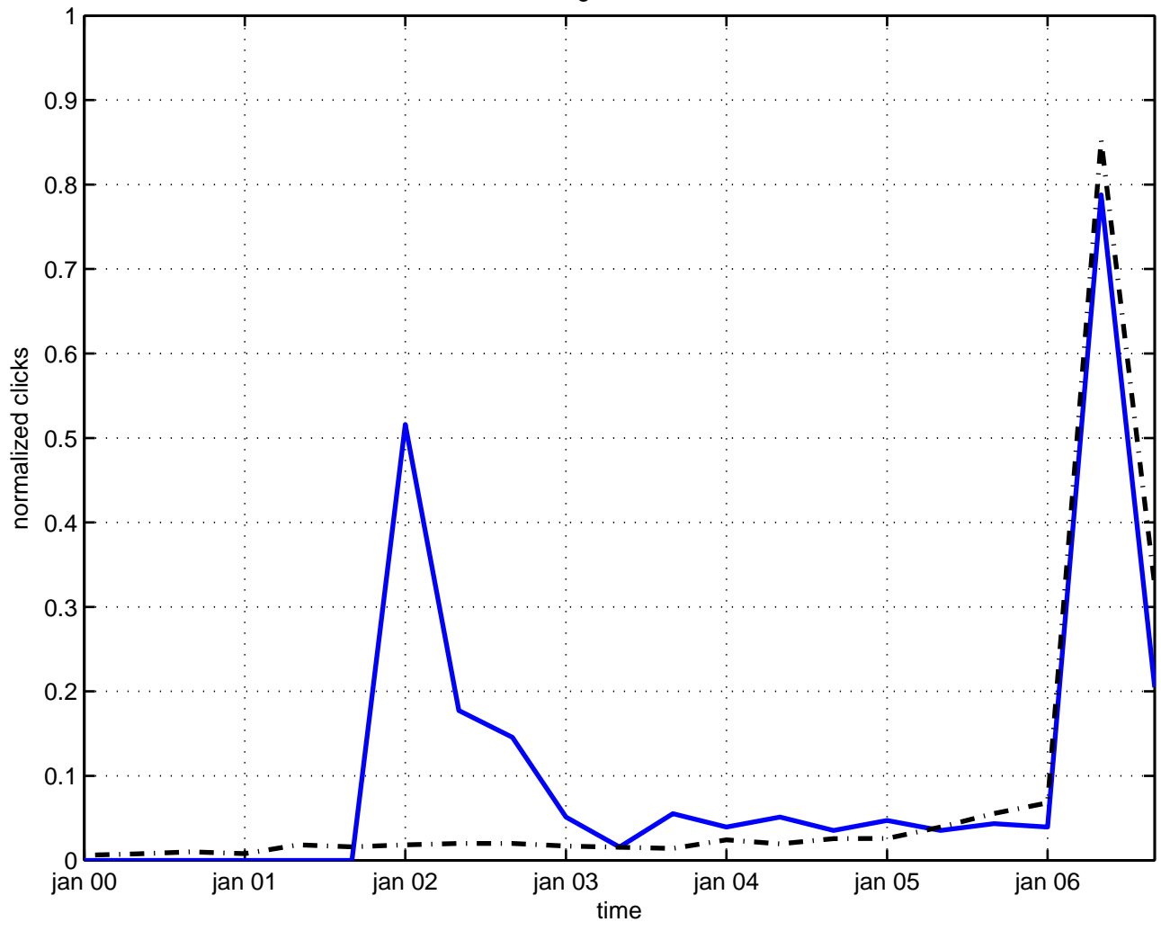
charge instanton
