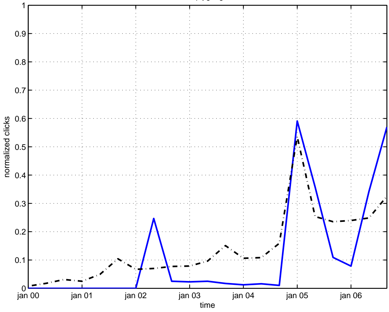
chaplygin gas
