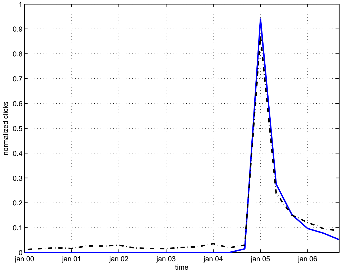
chaos critical phenomena
