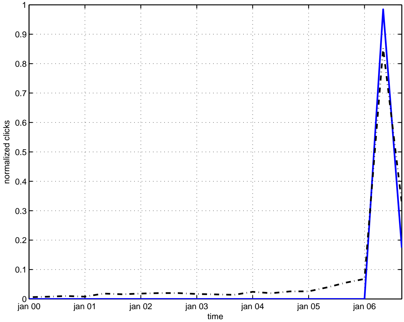
chain monopole
