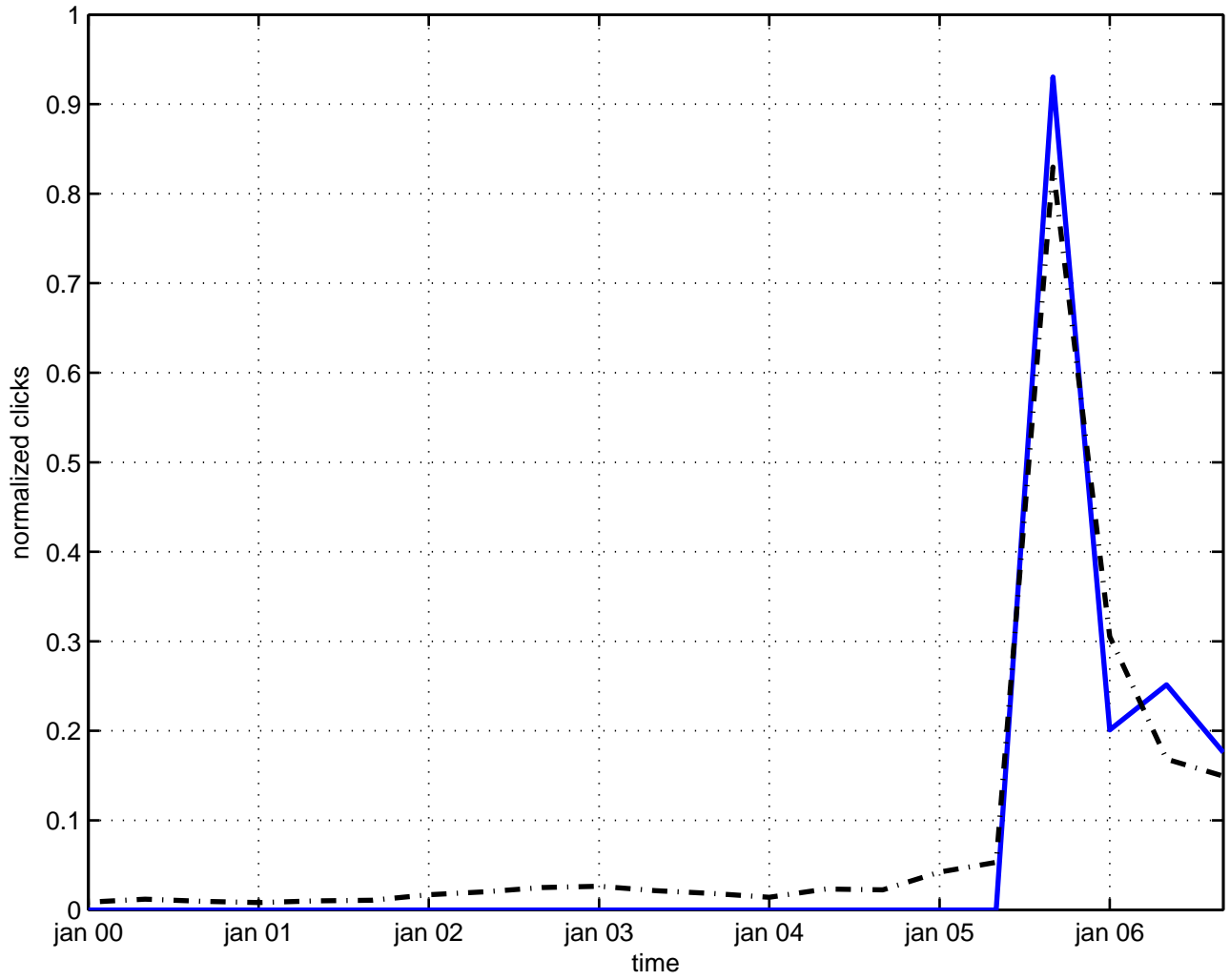
causality operator
