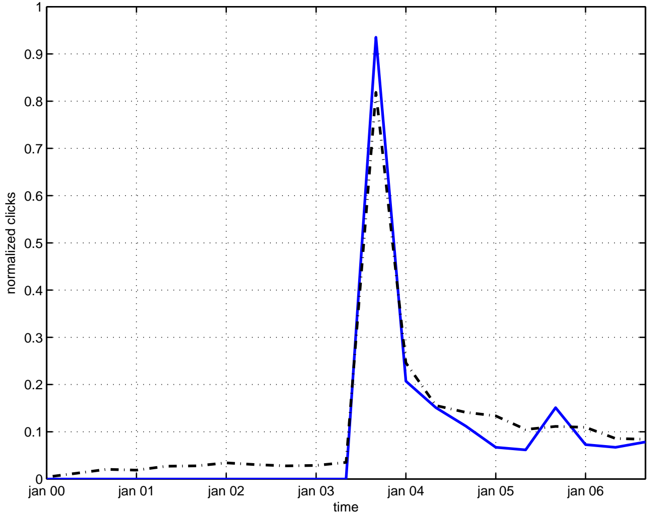
category tensor
