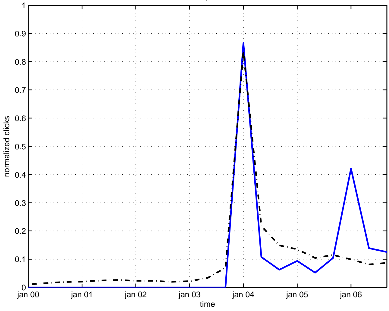
casimir pressure
