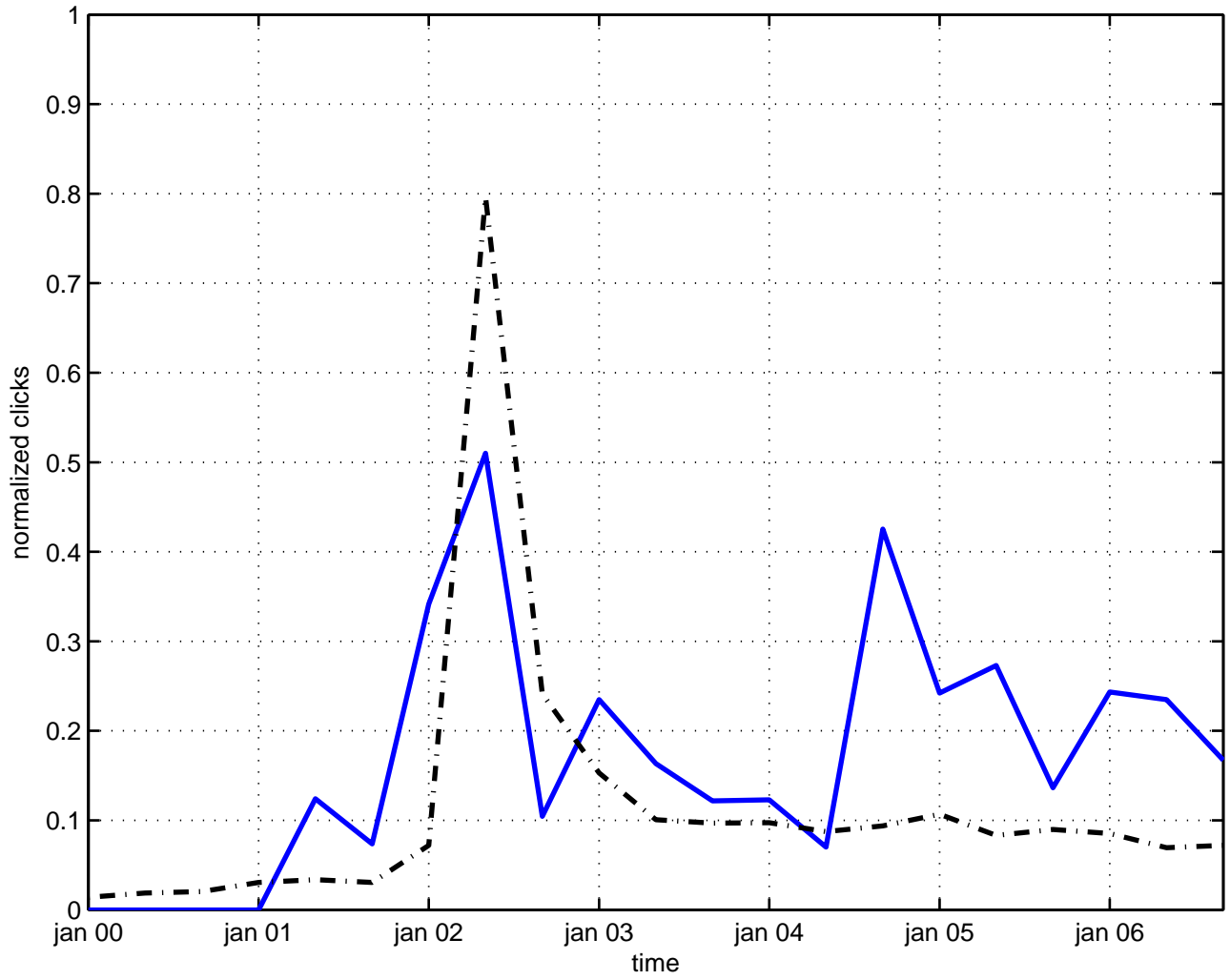
casimir operator
