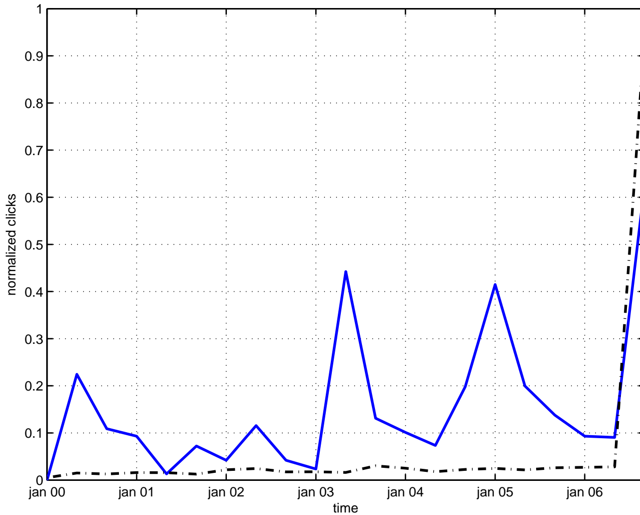
casimir force
