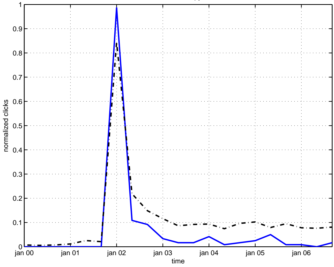
casimir entropy
