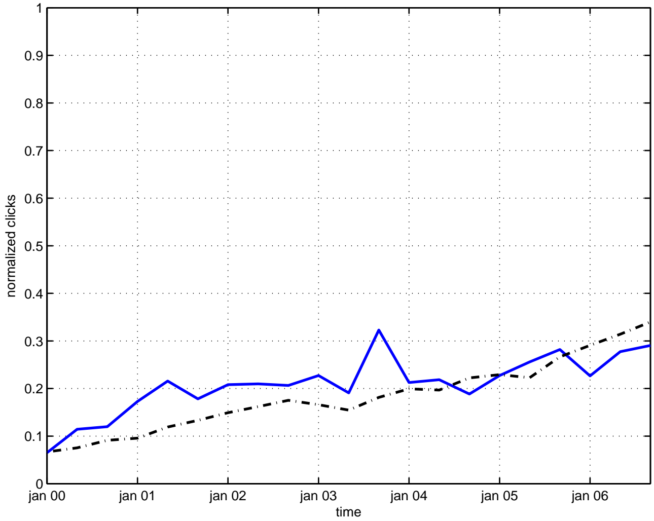
casimir energy
