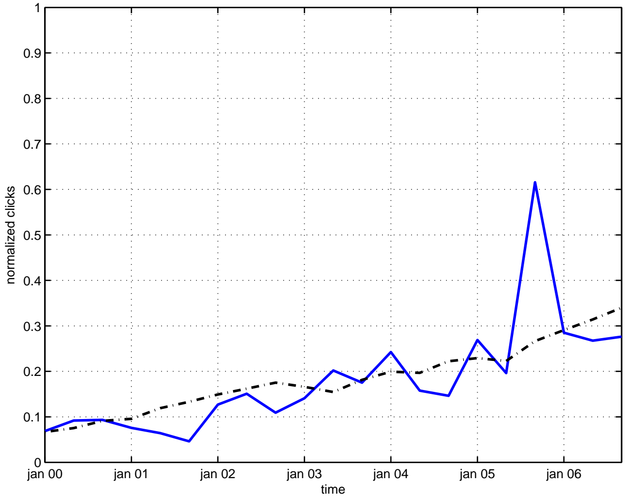
casimir effect
