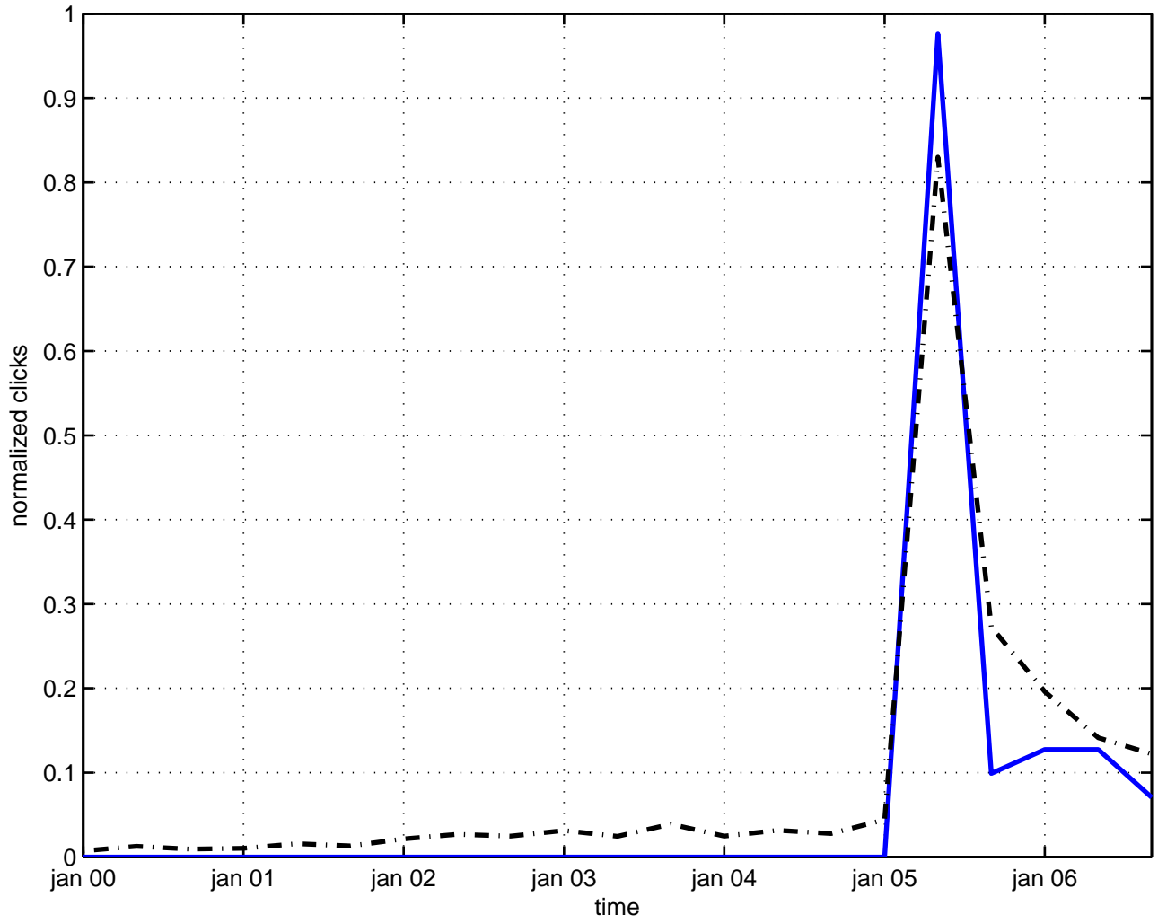
casimir density
