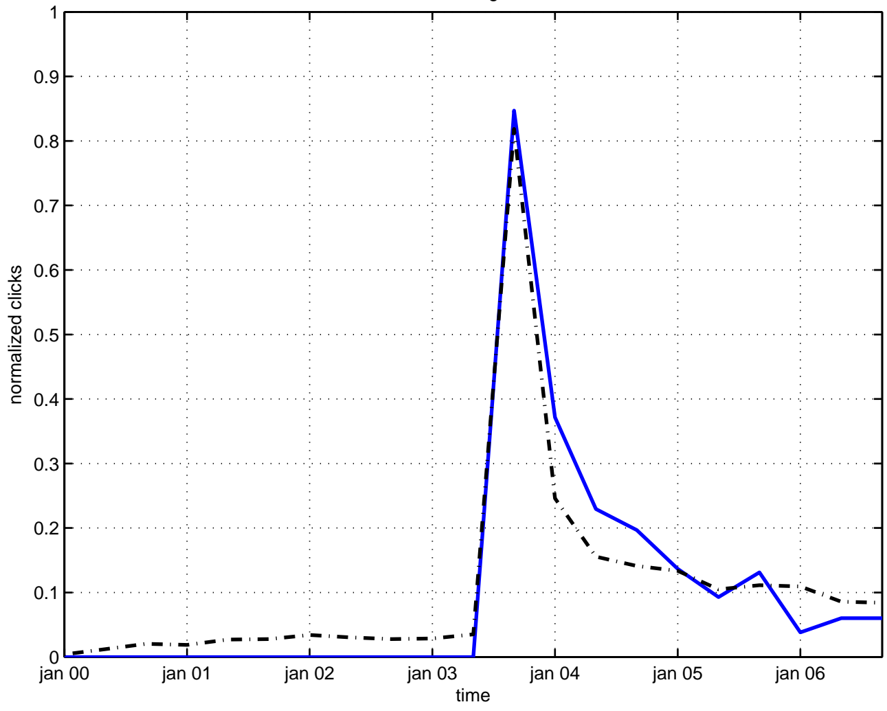
casimir algebra
