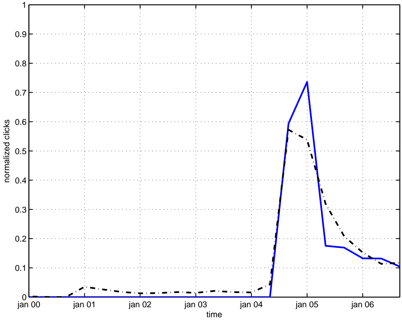
cargese 2004/06/07 talk
