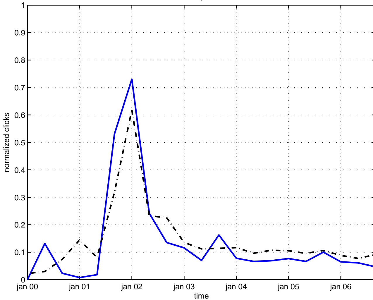
canonical quantization
