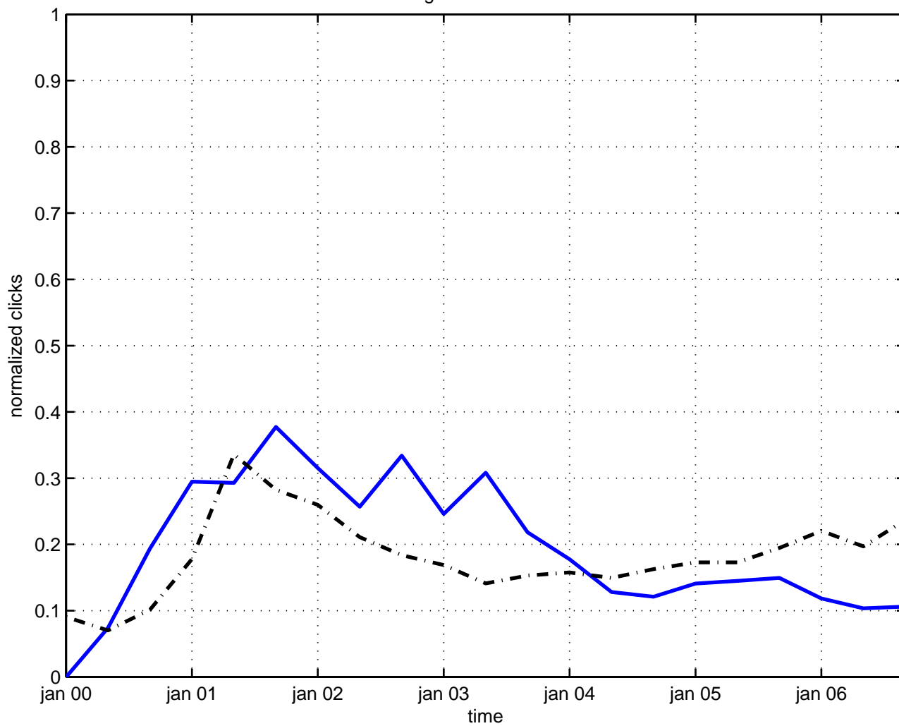
calogero-moser model
