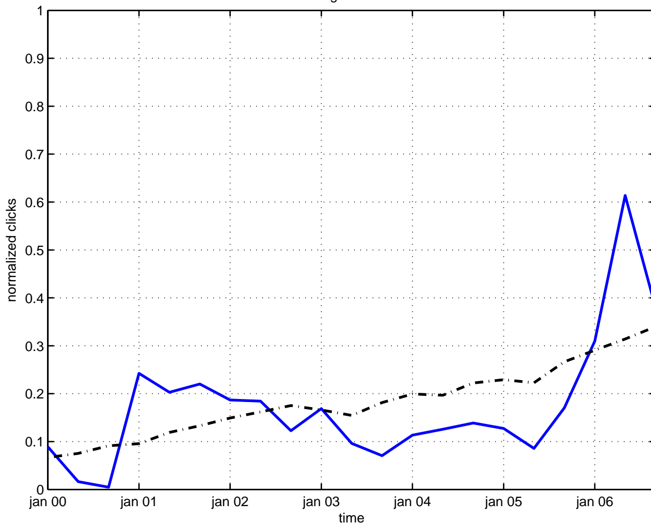
calogero model
