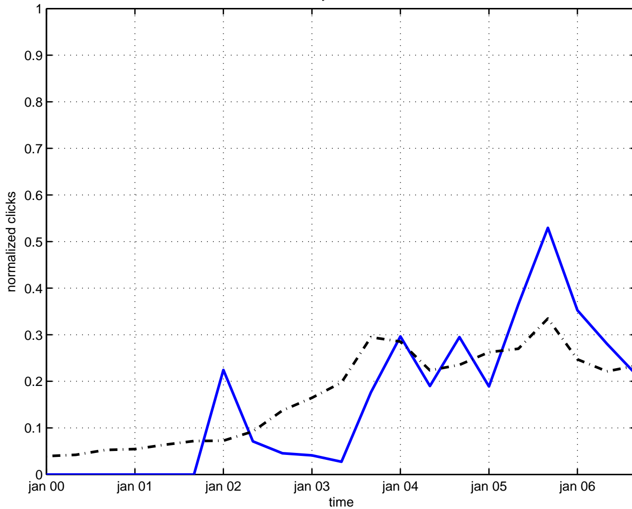
calabi-yau orientifold
