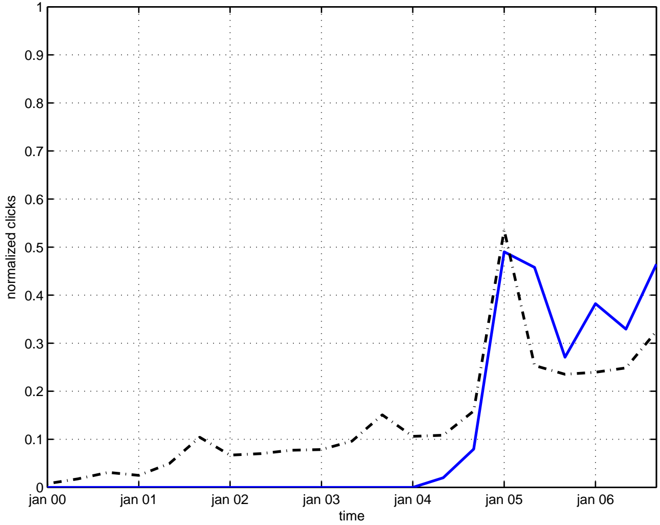
calabi-yau compactification
