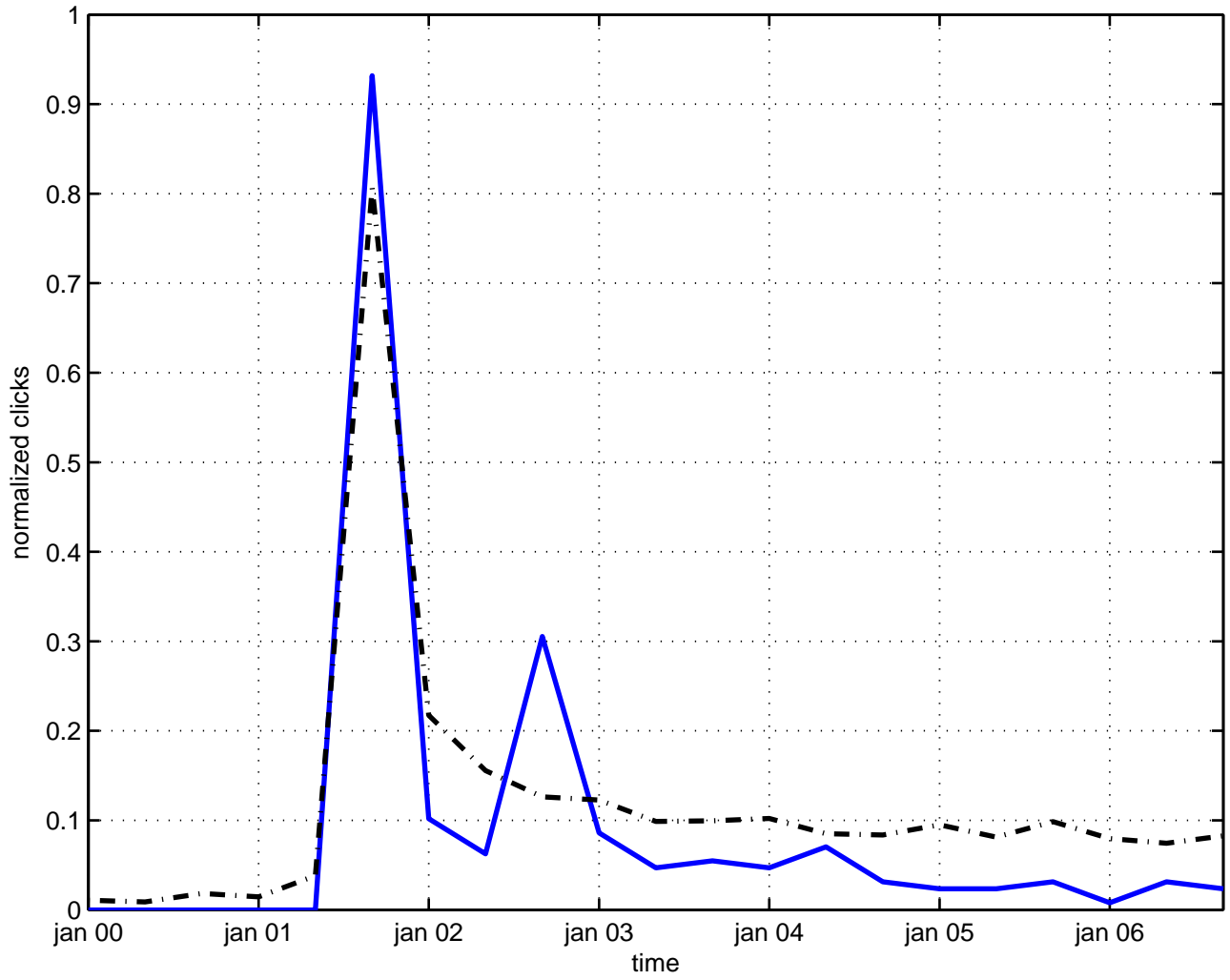
c-function renormalization
