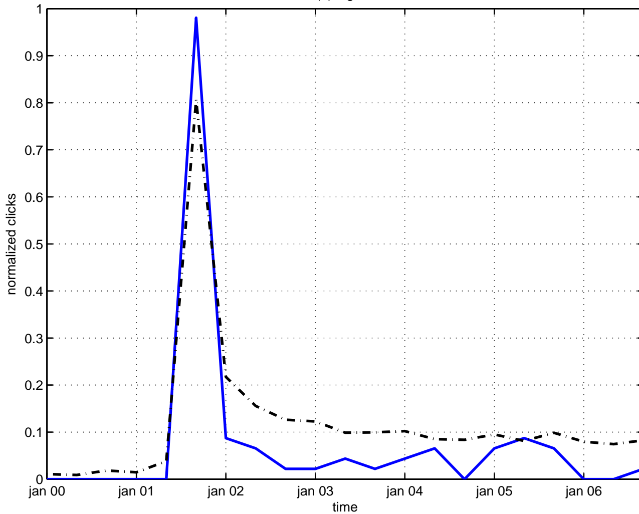
c(2) algebra
