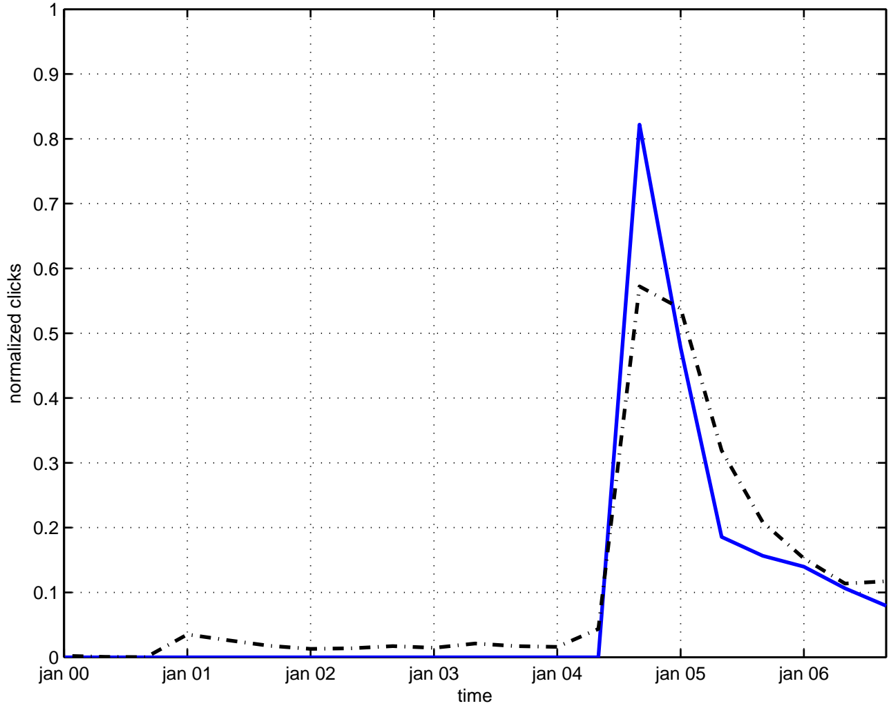
burst gravitational radiation
