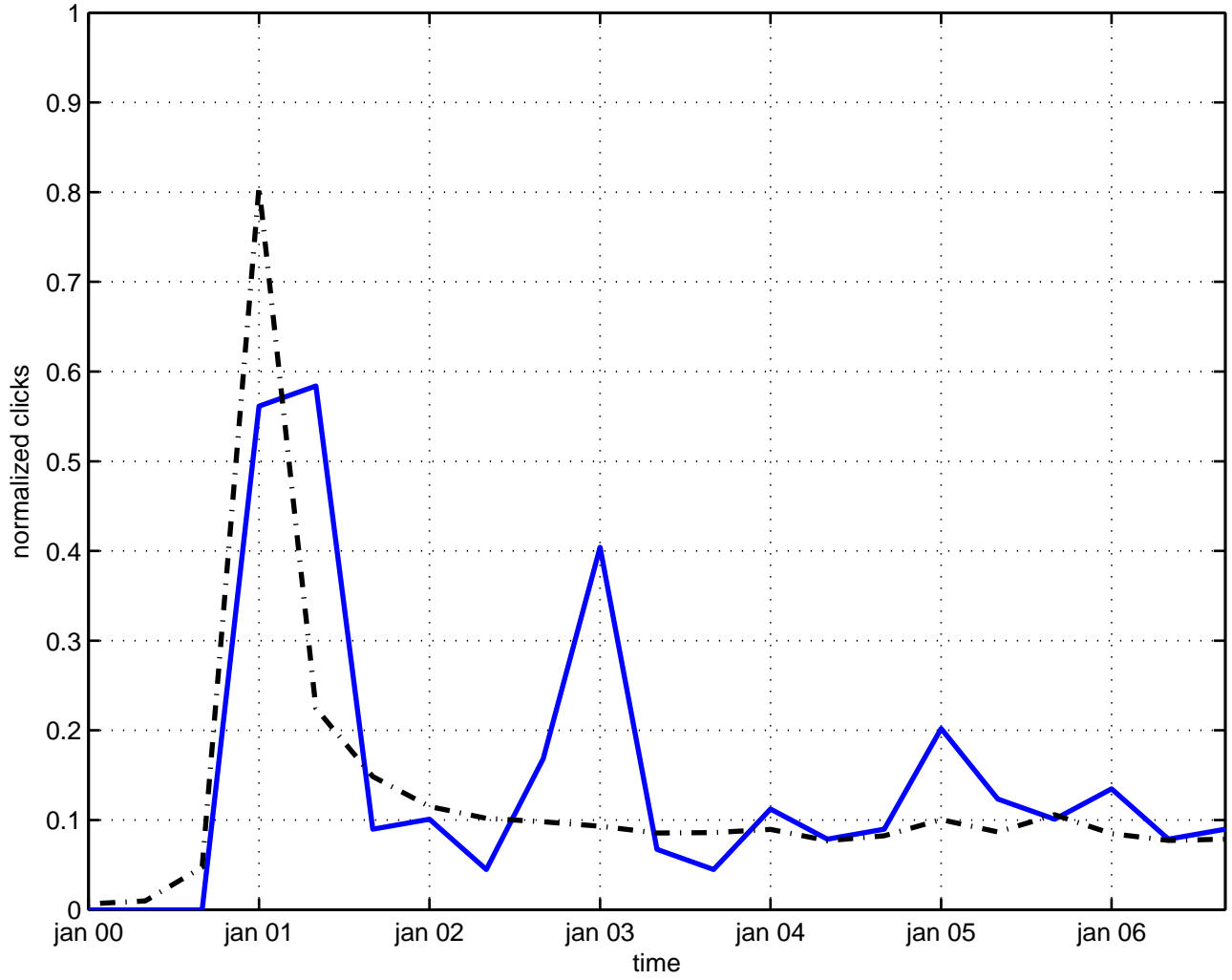
bullough-dodd model
