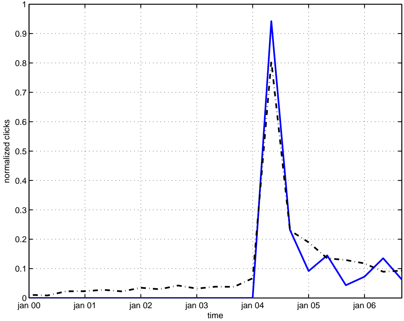
bubble kaluza-klein model
