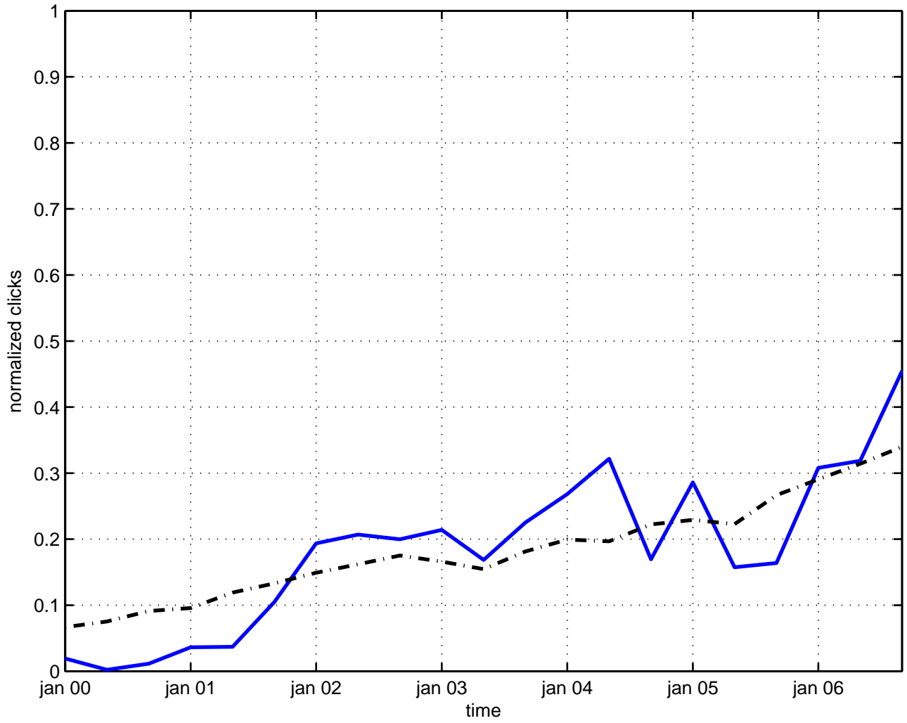
btz black hole
