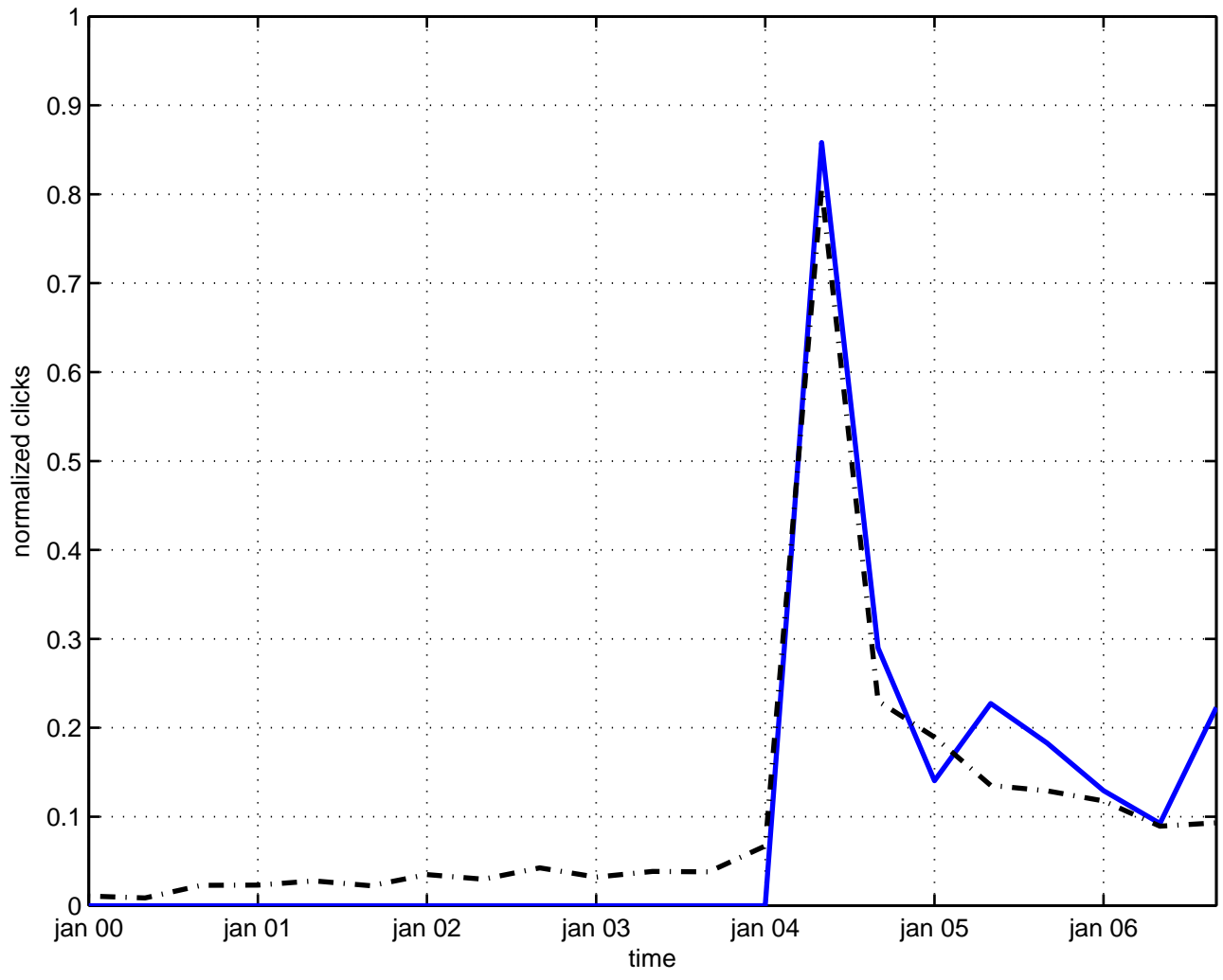
brownian motion
