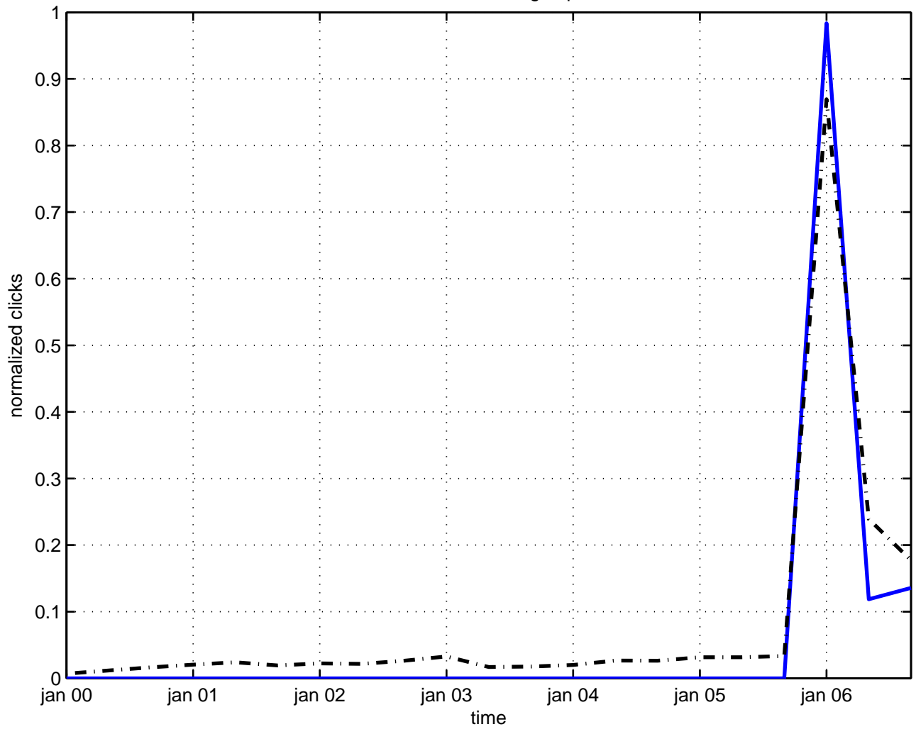
brownian motion charged particle
