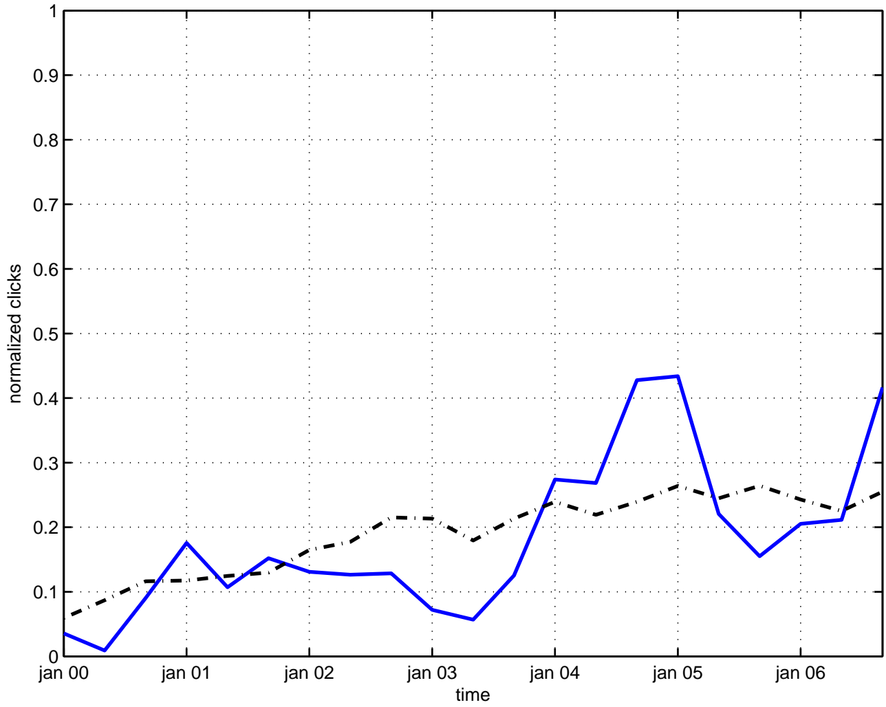
brans-dicke model
