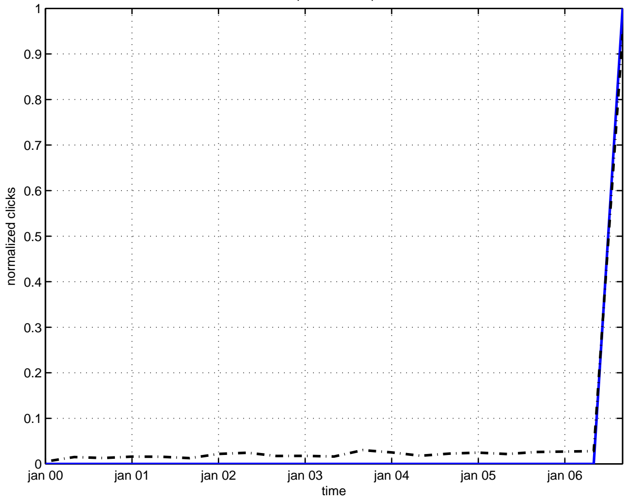
bps wilson loop
