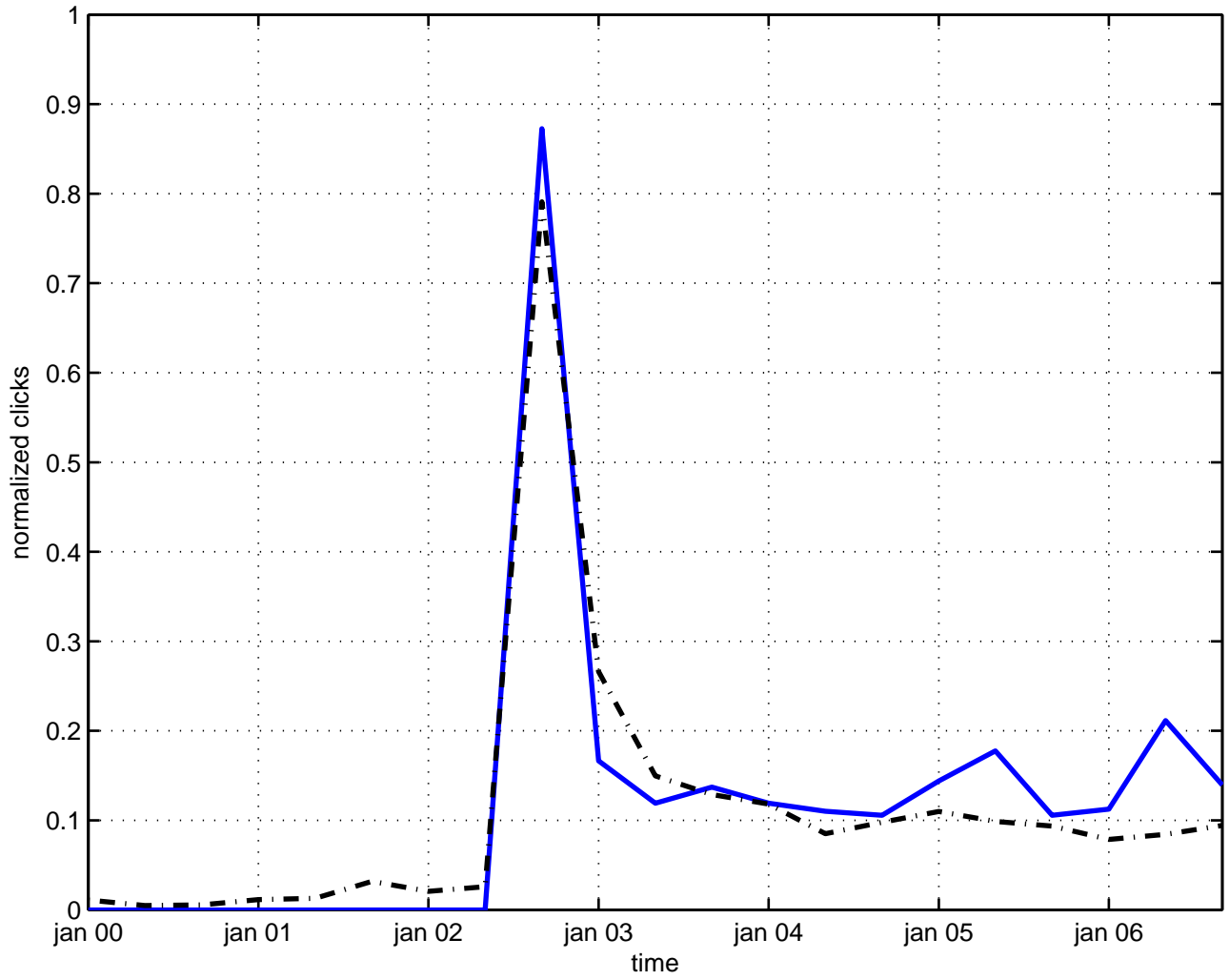
bps transformation
