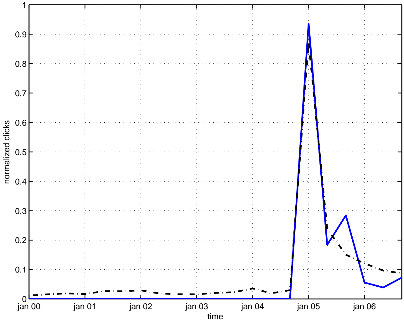
bps invariance
