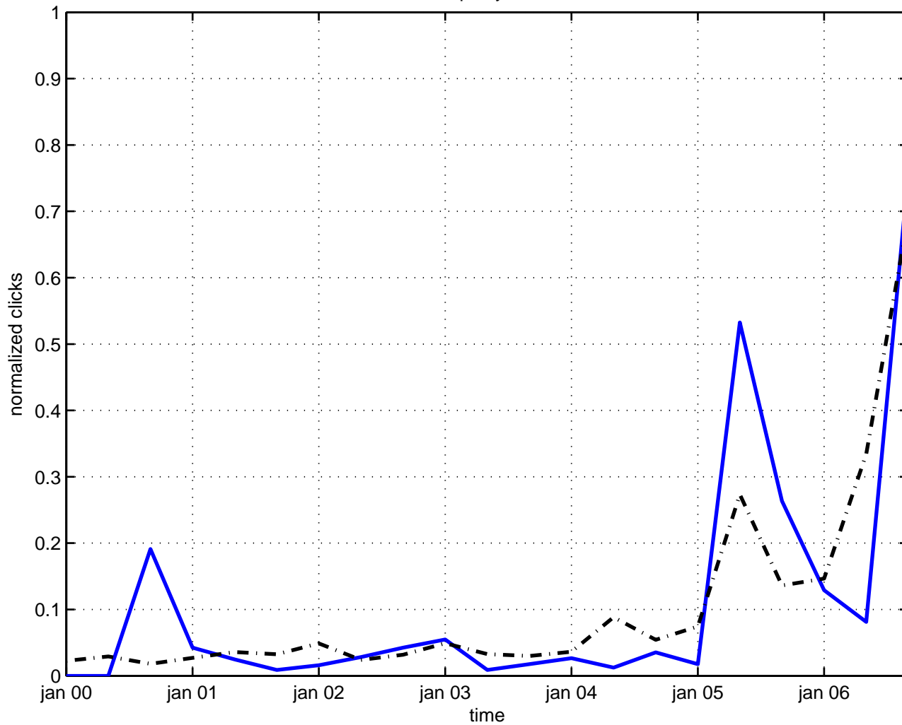
bps dyon
