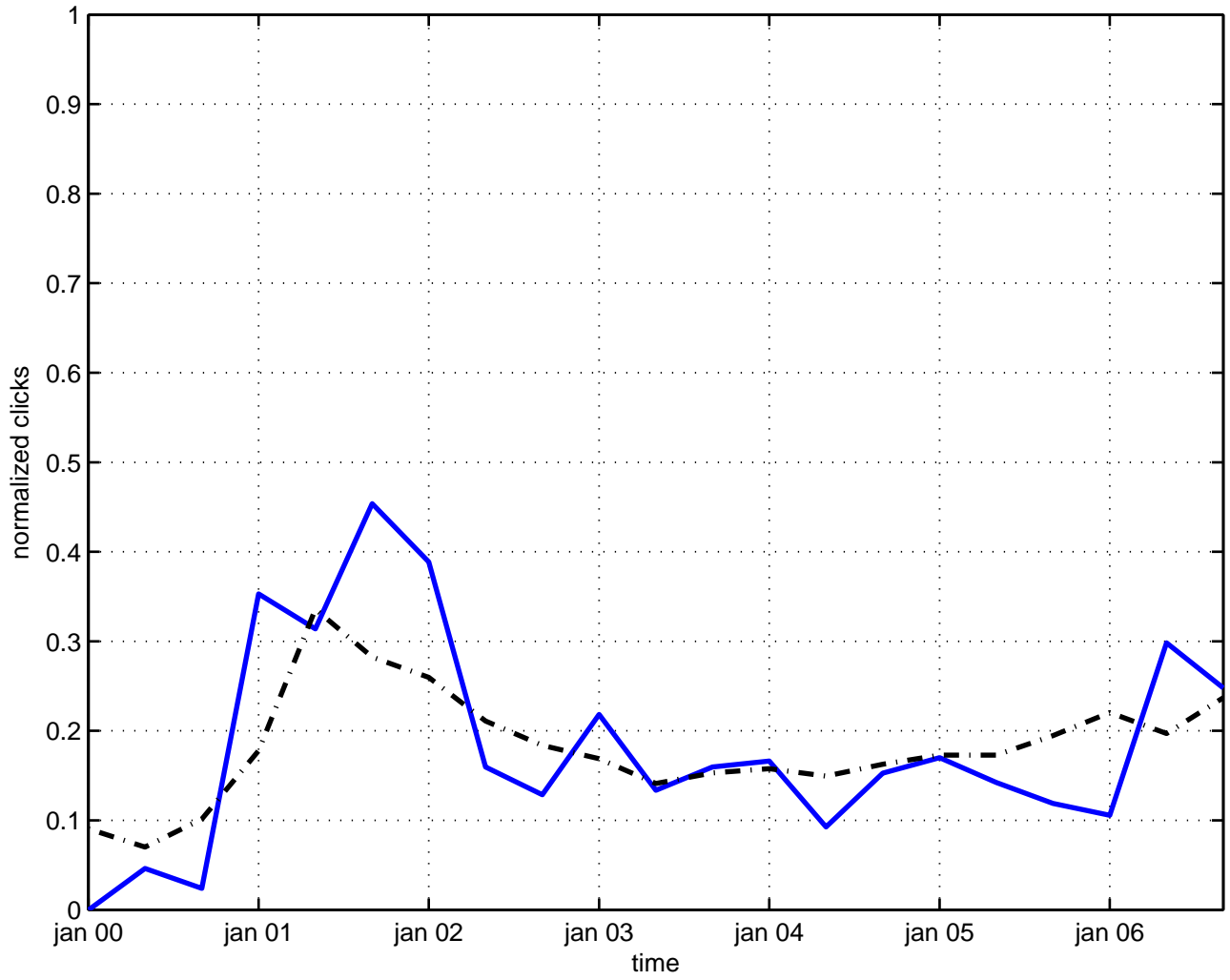
bps domain wall
