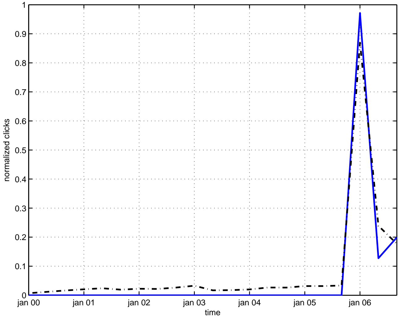
bps cosmic string
