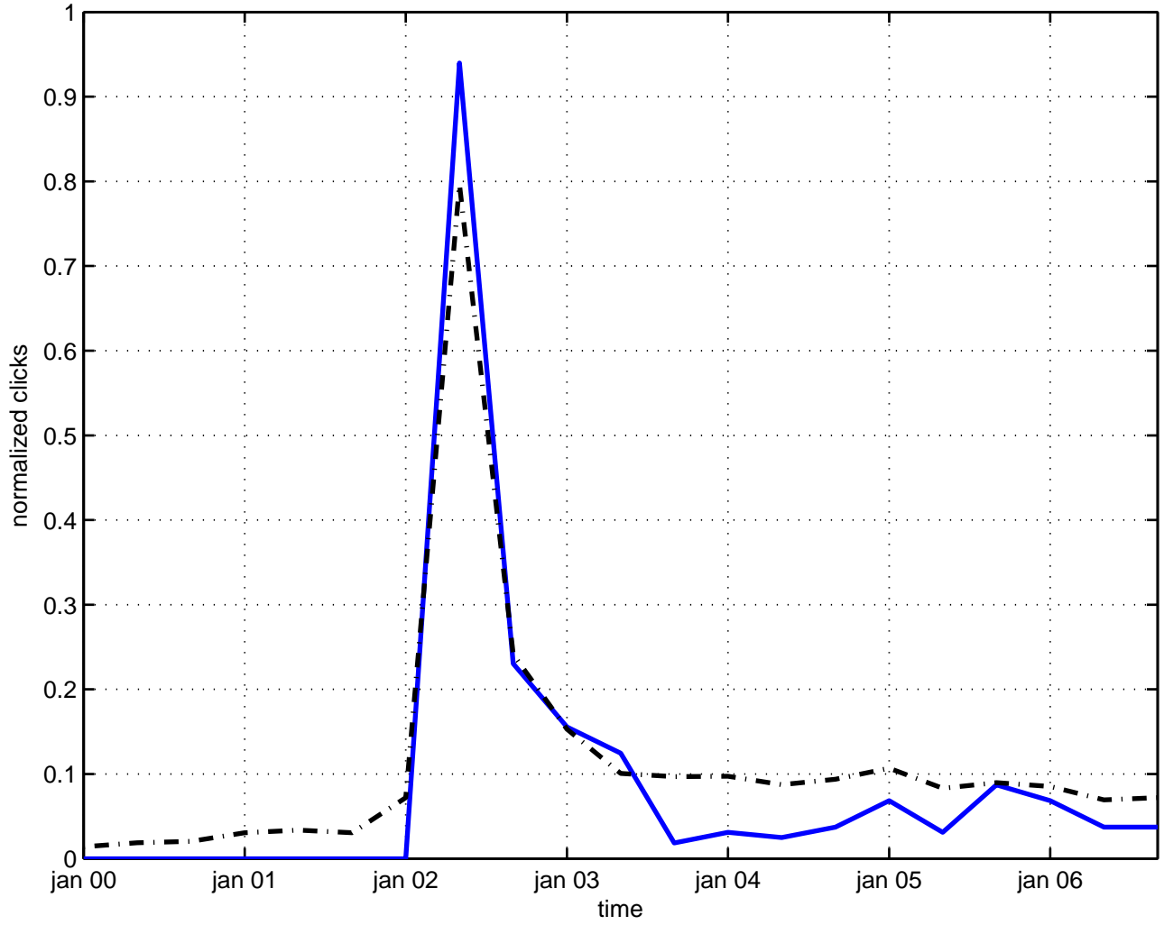
boundary condition quantum chromodynamics
