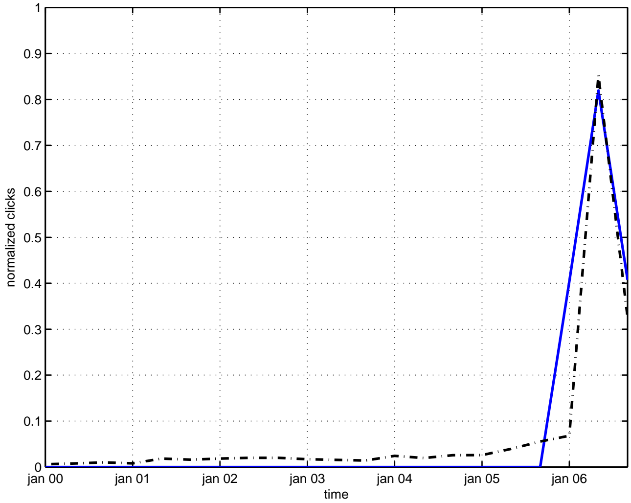
bound state magnon
